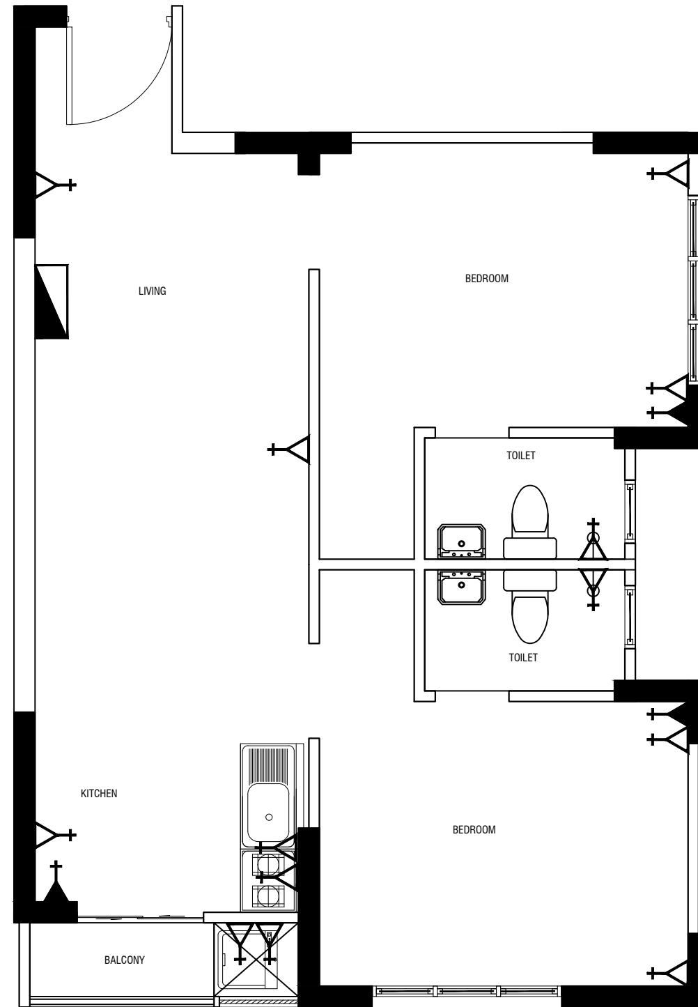
POWER LAYOUT (TYPE -2)
