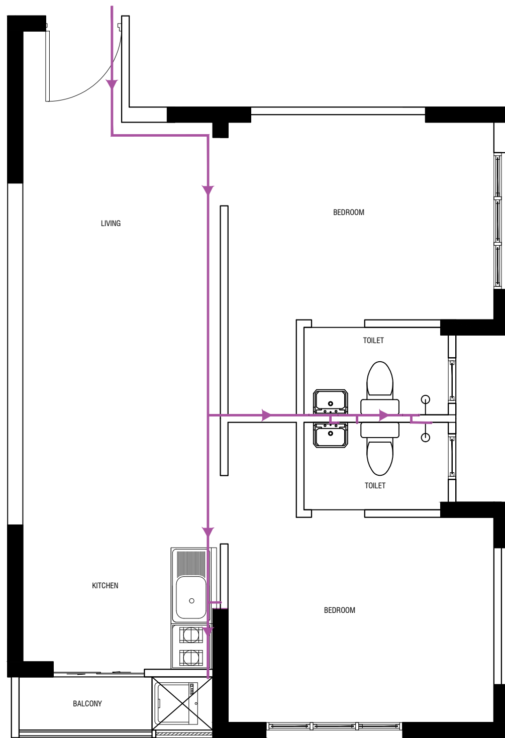
FRESH WATER SUPPLY - (TYPE-2)
