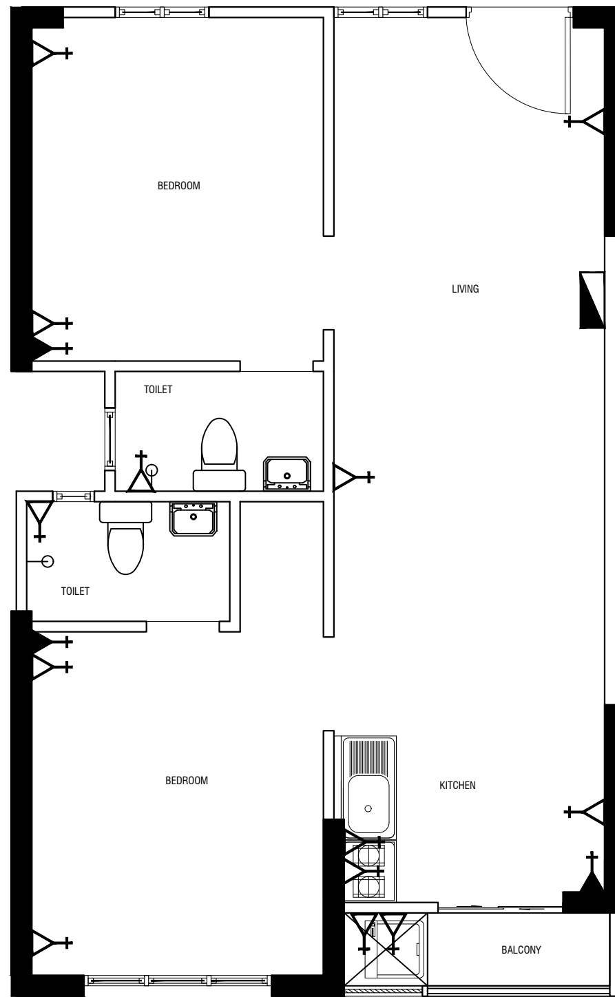
POWER LAYOUT (TYPE -1B)
