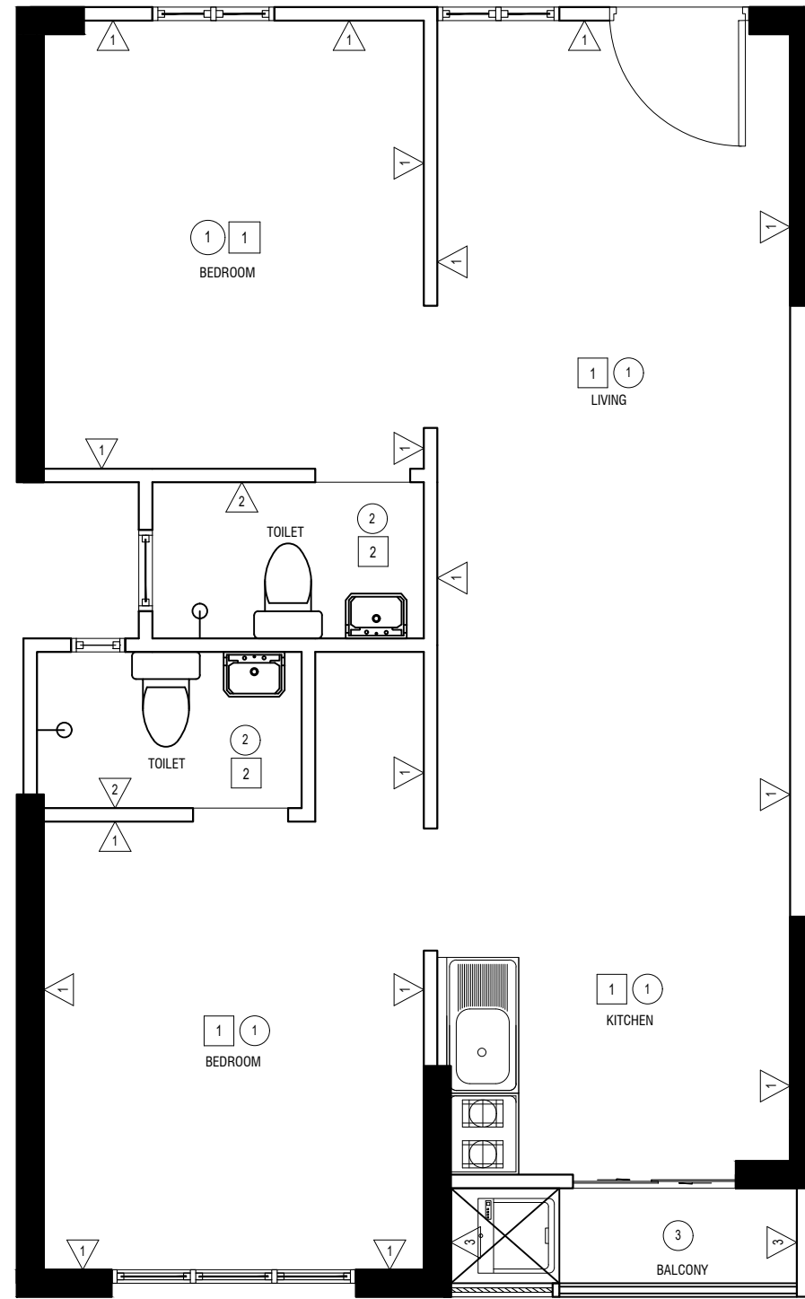
FINISHING SCHEDULE TYPE -1B SCALE 1:50
