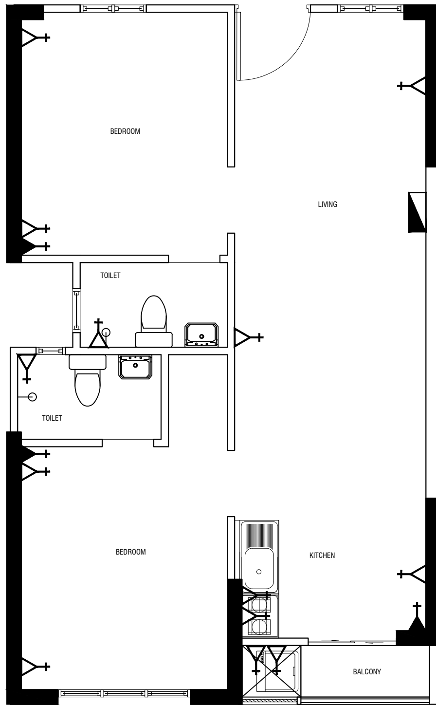
POWER LAYOUT (TYPE -1A) SCALE 1:50
