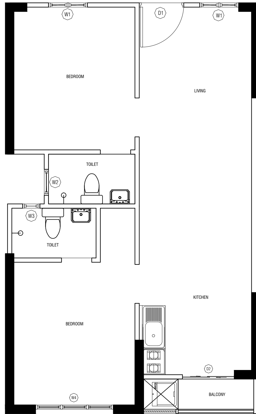
DOORS AND WINDOWS PLAN - (TYPE-1A) SCALE 1:50
