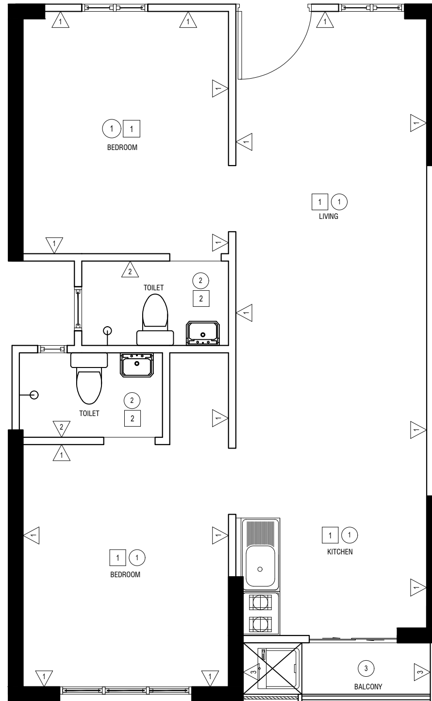
FINISHING SCHEDULE TYPE -1A SCALE 1:50
